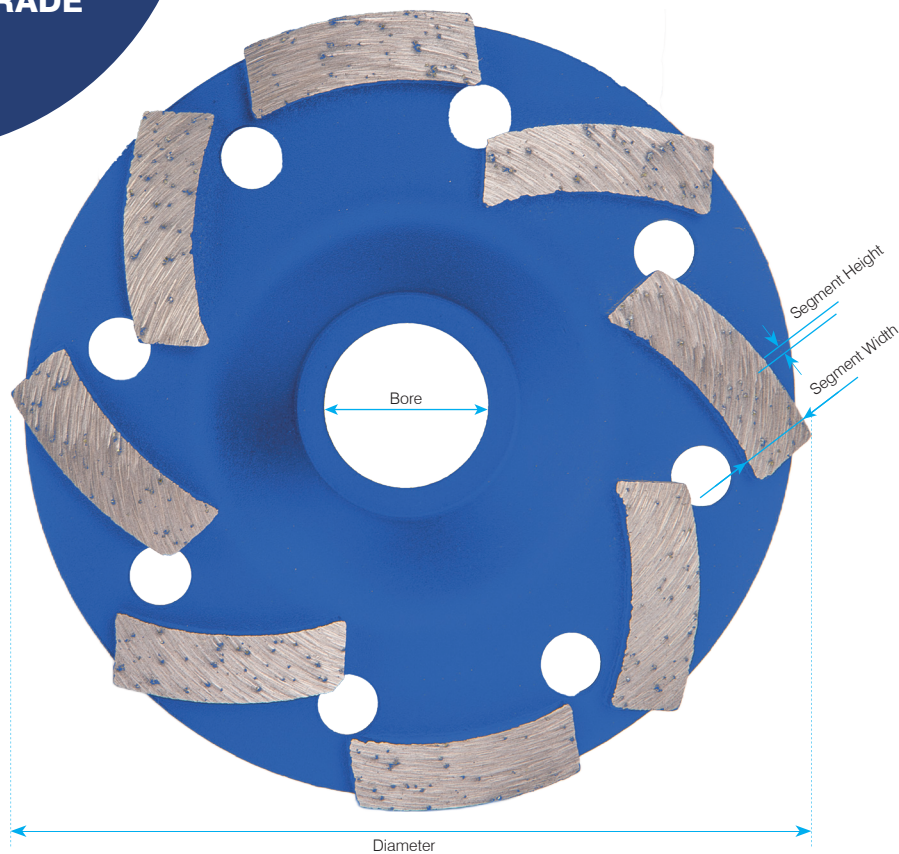
GM06-J-18005-TW ANGLE TEETH
